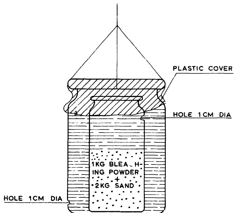
FIG.1 CHLORINATION POT FOR HOUSEHOLD WELLS CAP. 400 LITRES PER DAY (100 GPD) OF DRINKING WATER ; CHEMICAL RECHARGE EVERY 3 WEEKS (SOURCE : C PHERI , NAGPUR , INDIA)
